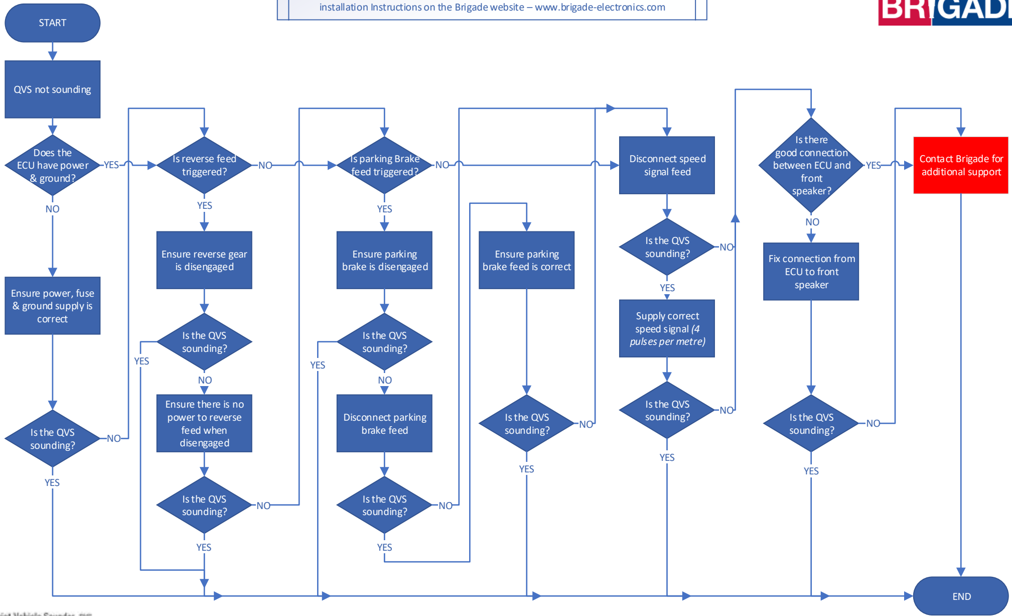
Quiet Vehicle Sounder QVS
